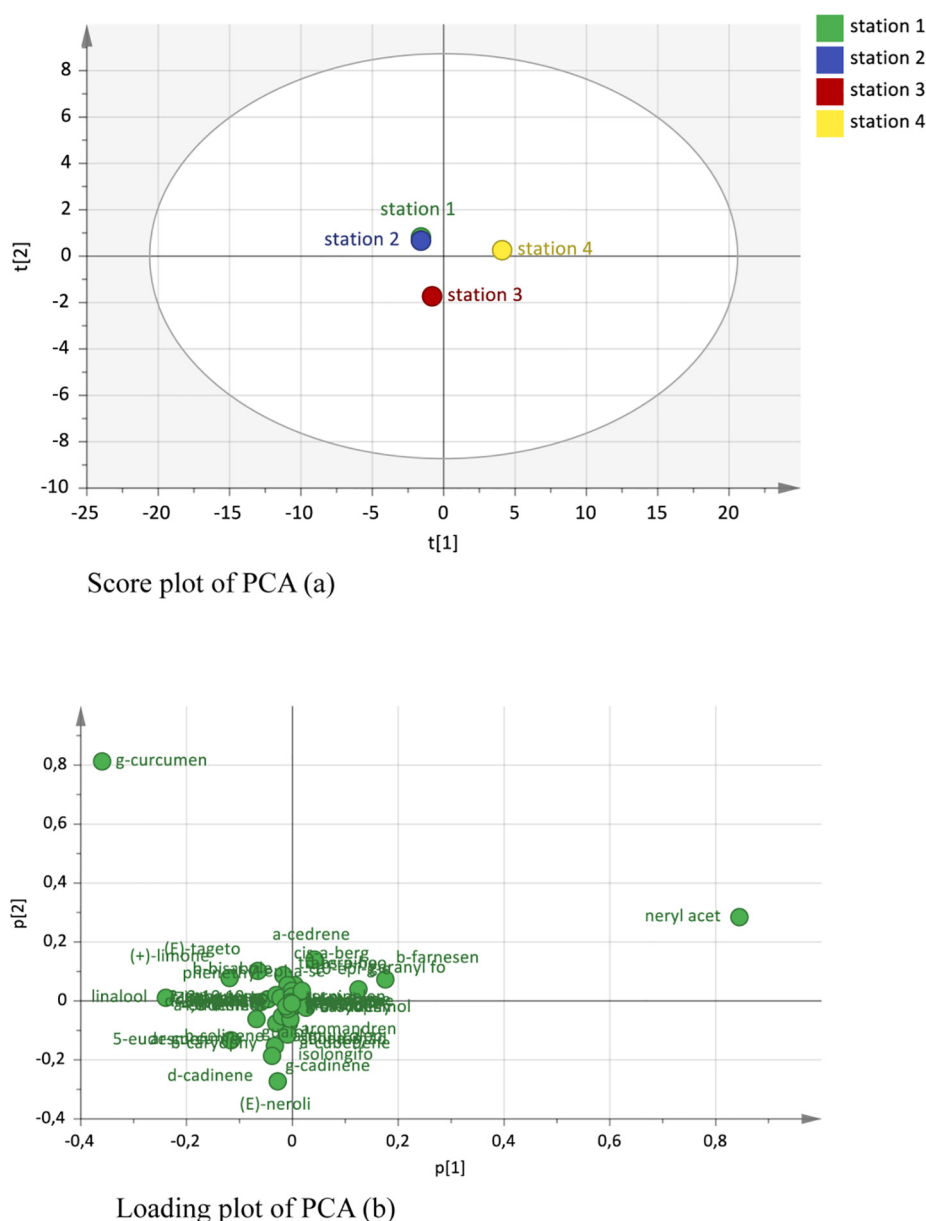
Fig. 2. PCA analysis and loading plot of PCA of essential oil of listed H. microphyllum subsp. tyrrhenicum samples.
