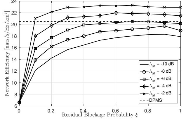
Fig. 5. Network spectral efficiency as a function of \xi . Here, the D2D pairs density is \lambda_D = 5\lambda_V .
