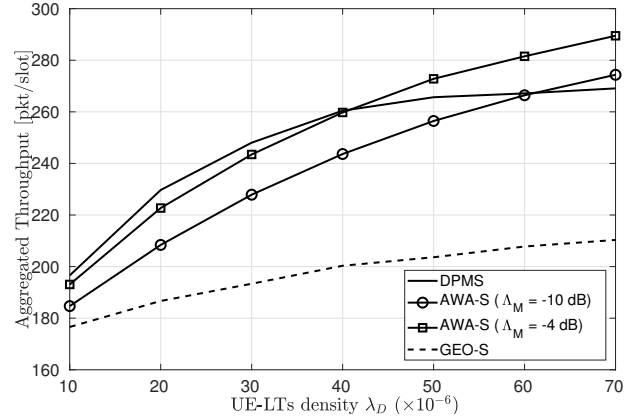
Fig. 7. Aggregated throughput, as a function of the UE-LTs density \lambda_D .
