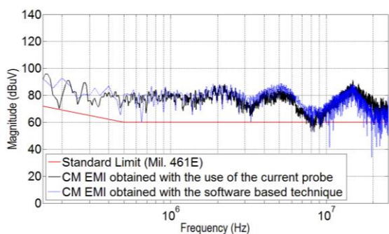
Fig. 6. Comparison between CM EMI obtained by the software-based separation technique and by RF measurement-based technique.
