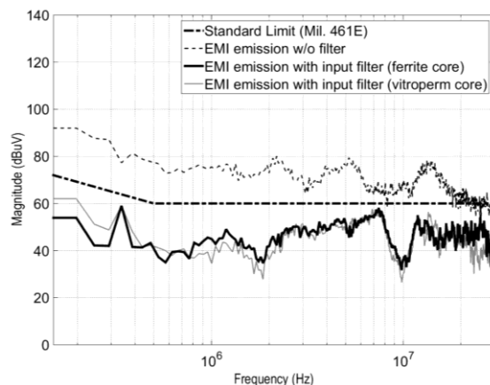
Fig. 13. Measured EMI emission without and with EMI filter.
