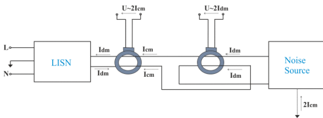
Fig. 4. Separation of CM and DM current by using a current probe.
