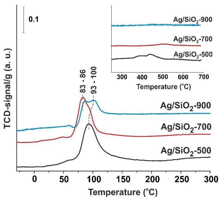
Fig. 11. TPSR-CO profiles (CO 2 desorption traces) for Ag/SiO 2 samples (5 wt. %) after adsorption of CO at -70 °C
