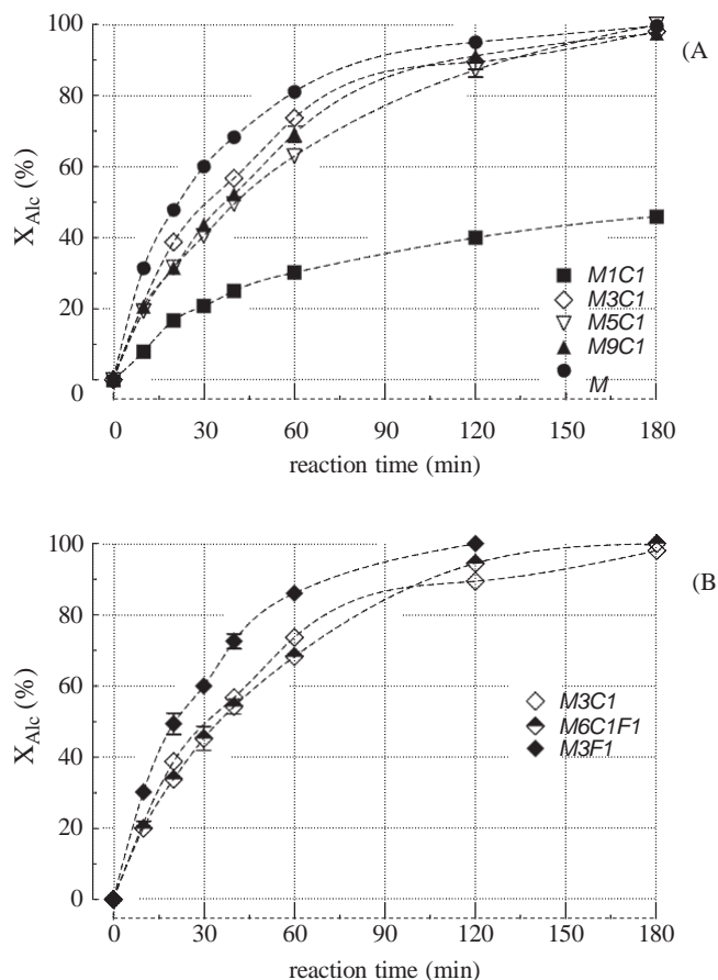
Fig. 8. Selective oxidation of benzyl alcohol on Ce (A) and Fe (B) promoted MnO x catalysts: conversion vs. reaction time ( T , 343K; V , 50 mL; V_{Alc} , 0.5 mL (4.86 mmol)); w_{cat} , 0.45g; F_{O_2} , 60 mL/min; P , 1 atm).
