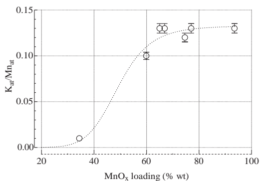
Fig. 1. Influence of the loading on the atomic K/Mn ratio of bare and promoted \text{MnO}_x catalysts.
