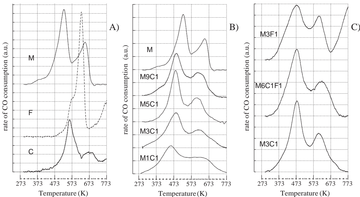
Fig. 5. CO-TPR profiles of: (A) bare C, F and M oxides; (B) Ce-promoted catalysts; and (C) M3C1, M6C1F1 and M3F1 catalysts (profiles in (B) and (C) normalized to the MnO_x content).
