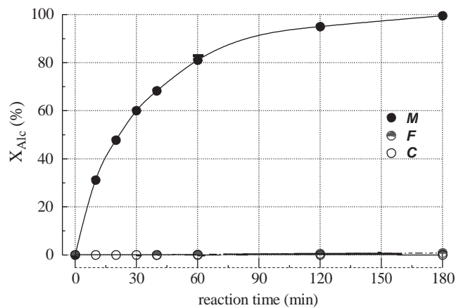
Fig. 6. Selective oxidation of benzyl alcohol on the bulk M, C and F systems: conversion vs. reaction time ( T , 343K; V , 50 mL; V_{Alc} , 0.5 mL (4.86 mmol); w_{cat} , 0.45 g; F_{O_2} , 60 mL/min; P , 1 atm).
