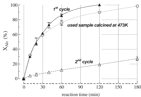
Fig. 11. Activity data of the M3C1 catalyst in the 1st and 2nd reaction cycles, and after calcination of the used sample (from 1st cycle) at 473 K.
