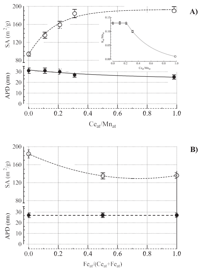
Fig. 2. (A) Influence of the atomic Ce/Mn ratio ( x/y ) on surface area (SA) and average pore diameter (APD) of \text{M}_x\text{C}_y catalysts; (B) Influence of the Ce and Fe content on SA and APD of the M3C1, M6C1F1 and M3F1 catalysts.
