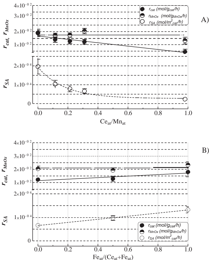
Fig. 9. Effect of the catalyst composition on the various specific initial rates: (A) influence of the Ce/Mn atomic ratio on the reactivity of Ce-promoted catalysts; and (B) influence of the Ce and Fe content on the reactivity of M3C1, M6C1F1 and M3F1 catalysts.
