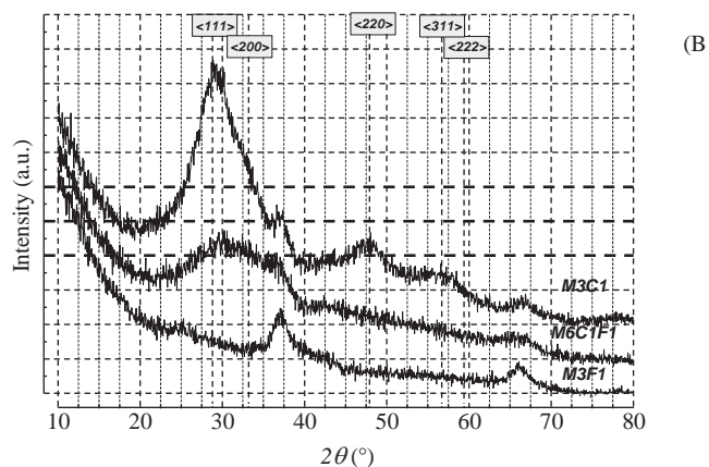
Fig. 3. XRD patterns of: (A) Ce-promoted catalysts; (B) M3C1, M6C1F1 and M3F1 catalysts. For reference the position of the main reflections of the cerianite habit are indicated.
