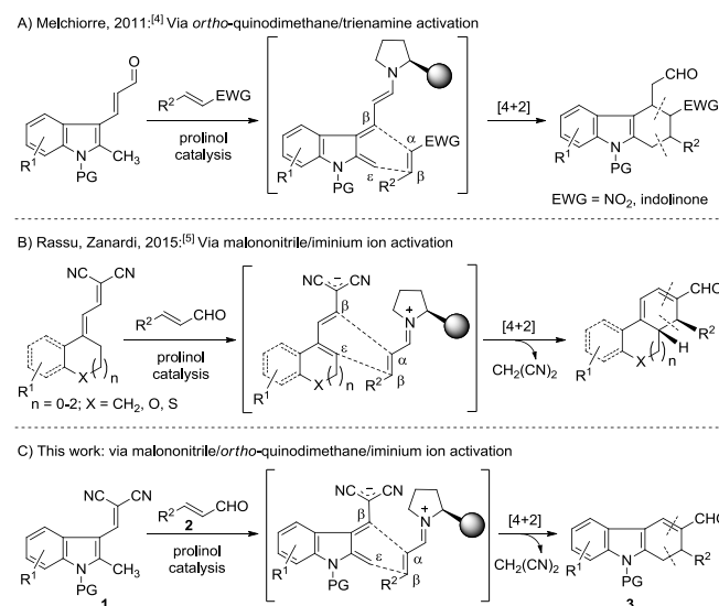
Scheme 1. Diarylprolinol silyl ether-catalyzed asymmetric [4+2] cycloaddition strategies.
