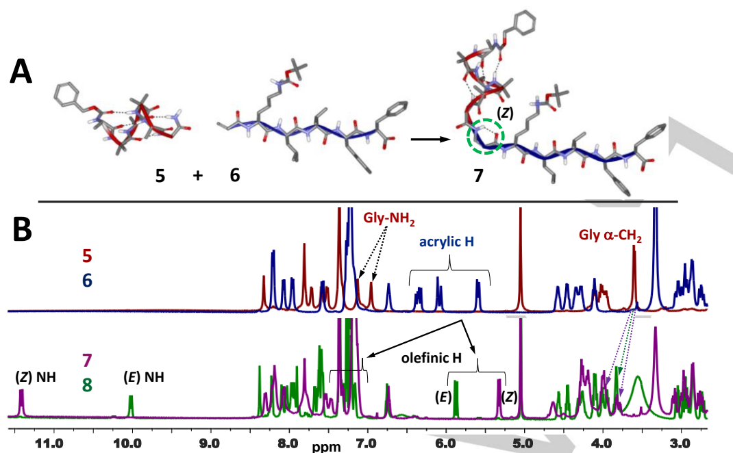
Figure 3. (A) Computer-generated model of Z-(Ala-Aib) _2 -Ala-Gly- \Delta^2\beta Ala-Lys (Boc) -Leu-Val-Phe-Phe-OH ( 7 ), which combines a helical domain (from 5 ) with a \beta -sheet promoting segment (from 6 ). The \Delta^2\beta Ala junction is circled. (B) Overlap of the ^1\text{H} NMR spectra (DMSO- d_6 ) of the two reactants (upper part, 5 , red trace, and 6 , blue trace) and (lower part) of the resulting product (Z) 7 (violet) and its E isomer 8 (green). Diagnostic signals are marked.
