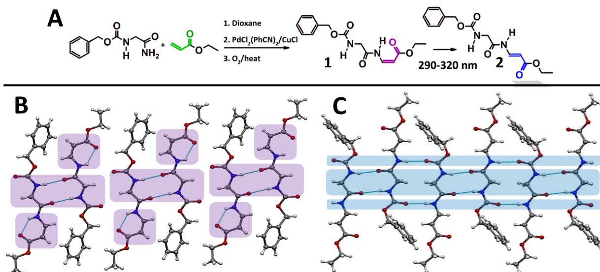
Figure 1. (A): Synthesis of Z-Gly- \Delta^2\beta Ala-OEt ( 1 ) and its photo-conversion to Z-Gly- \Delta^5\beta Ala-OEt ( 2 ). (B) and (C): Packing modes in the crystal structures of 1 and 2 , respectively. Intra- and intermolecular H-bonds are indicated by dashed lines.
