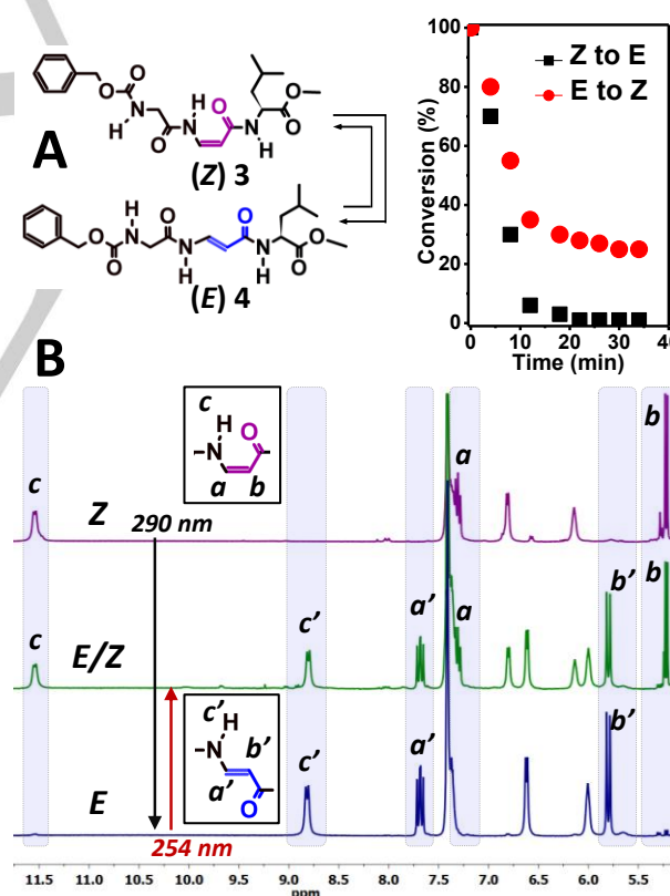
Figure 2. (A) Left: formulas of Z-Gly- \Delta^2\beta Ala-Leu-OMe ( 3 ) and Z-Gly- \Delta^5\beta Ala-Leu-OMe ( 4 ). Right: time evolution of their photo-conversions monitored by HPLC. (B) 1 H NMR spectra (CD 3 CN) of (Z) 3 (top), its (E) isomer 4 obtained by irradiation at 290-320 nm (bottom), and the mixture of E/Z isomers resulting as photo-stationary equilibrium upon irradiation of the E isomer at 254 nm (center). Diagnostic signals are marked. 3 J coupling constants between olefinic protons are 9 Hz for (Z) 3 and 14 Hz for (E) 4 .
