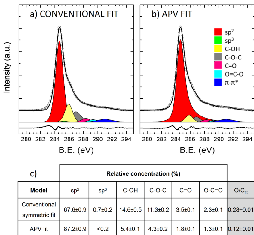
Fig. 4. C 1s spectra of RGO ( T_{\text{ann}} = 600^{\circ}\text{C} ). a) Conventional symmetric Voigt fit; b) APV fit. Shirley background was subtracted and an offset added. The \text{O}/\text{C}_{\text{area}} was 0.107 \pm 0.002 . The table reports the precise abundancy (in %) of the different chemical species, obtained with the two fitting protocols.
