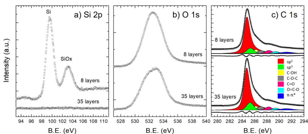
Fig. 6. XPS spectra a) Si 2p, b) O 1s and c) APV deconvolution of C 1s of the RGO ( T_{\text{ann}} = 300^\circ\text{C} ) with two thicknesses: 8 \pm 1 ( O/C_{\text{fit}} = 0.20 \pm 0.01 ) and 35 \pm 2 ( O/C_{\text{fit}} = 0.18 \pm 0.01 ) layers. The Si 2p signal was not detectable on the 35-layer films.
