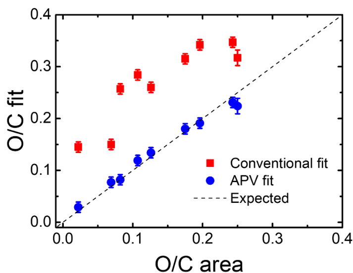
Fig. 5. Correlation plot: \text{O}/\text{C}_{\text{fit}} vs. \text{O}/\text{C}_{\text{area}} . Values obtained from analysis of XPS data from our samples using the conventional symmetric model (■), as in the standard literature approach, and the APV fit (●) developed here. The dotted line corresponds to perfect, ideal correlation.
